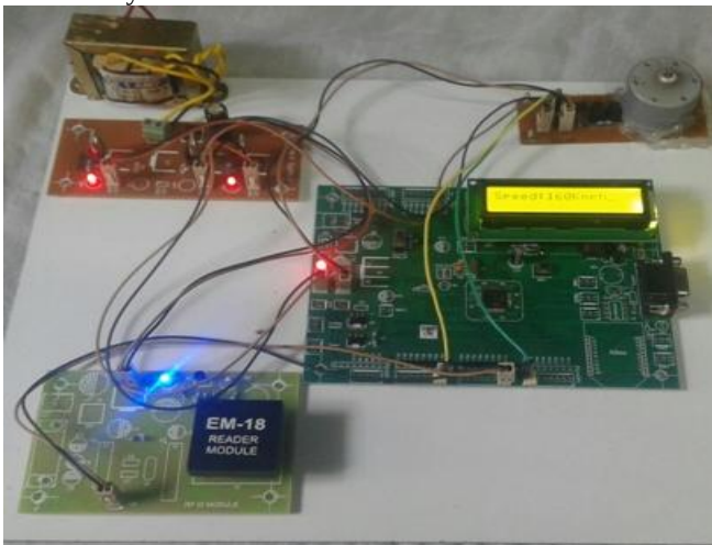
Fig 2.RFID and vehicle system is on.
