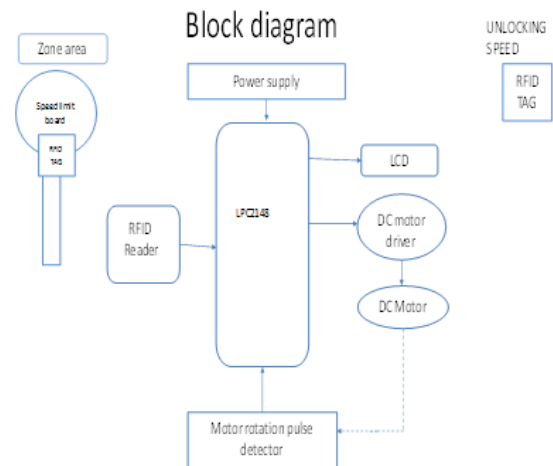
Fig1.Block Diagram.
